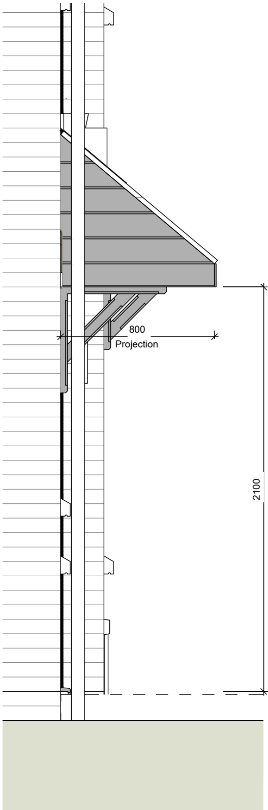
2 Gable Elevation 1 : 20
